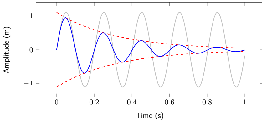
Figure: Under-damped system. IC: x_0 = 0 , \dot{x}_0 = 1e - 4
