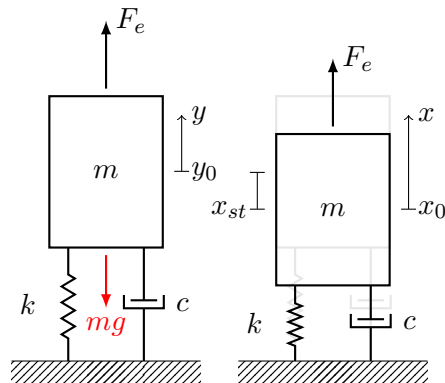
Figure: Mass-spring-damper system under gravity.
