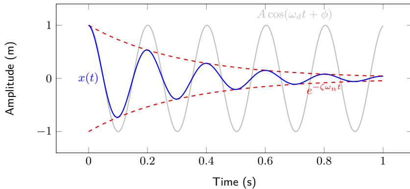
Figure: Under-damped system. IC: x_0 = 1 , \dot{x}_0 = 0
