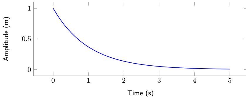
Figure: Displacement response due to initial displacement x_0 = 1 .
