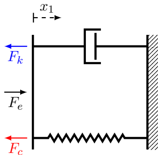
Figure: Fixed spring-dashpot system.
